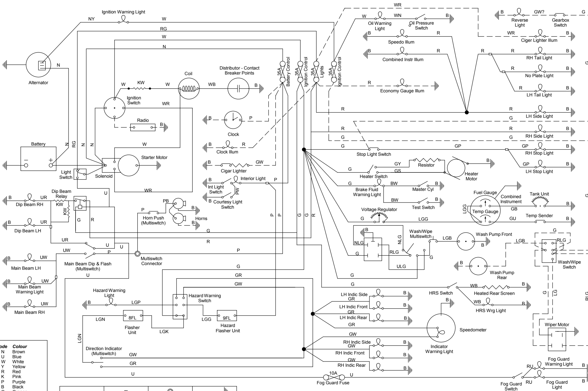
Reliant SE Wiring Diagram
