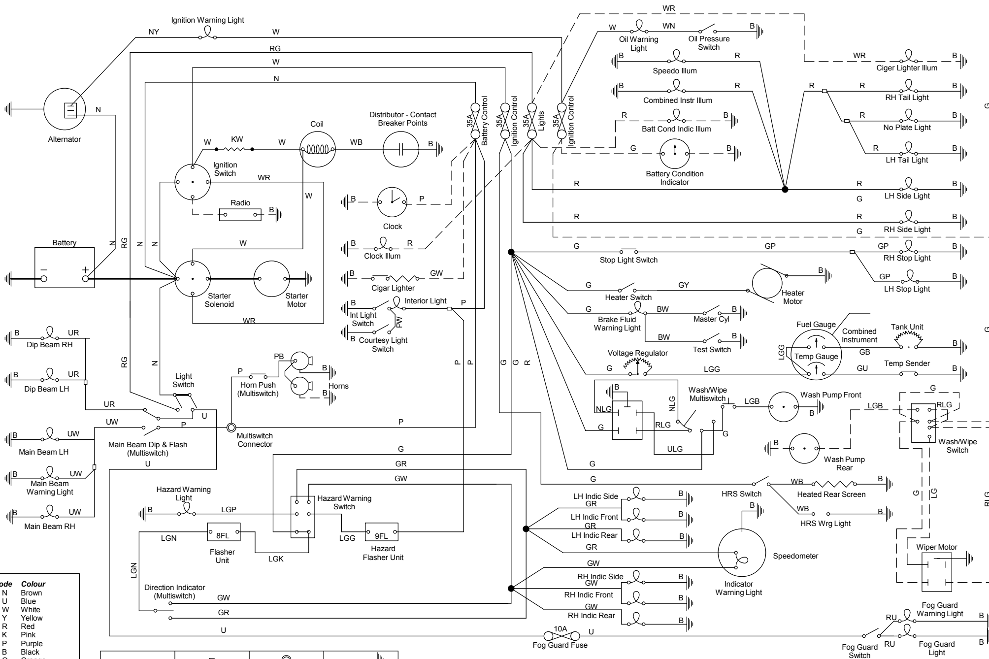
Rialto Wiring Diagram
