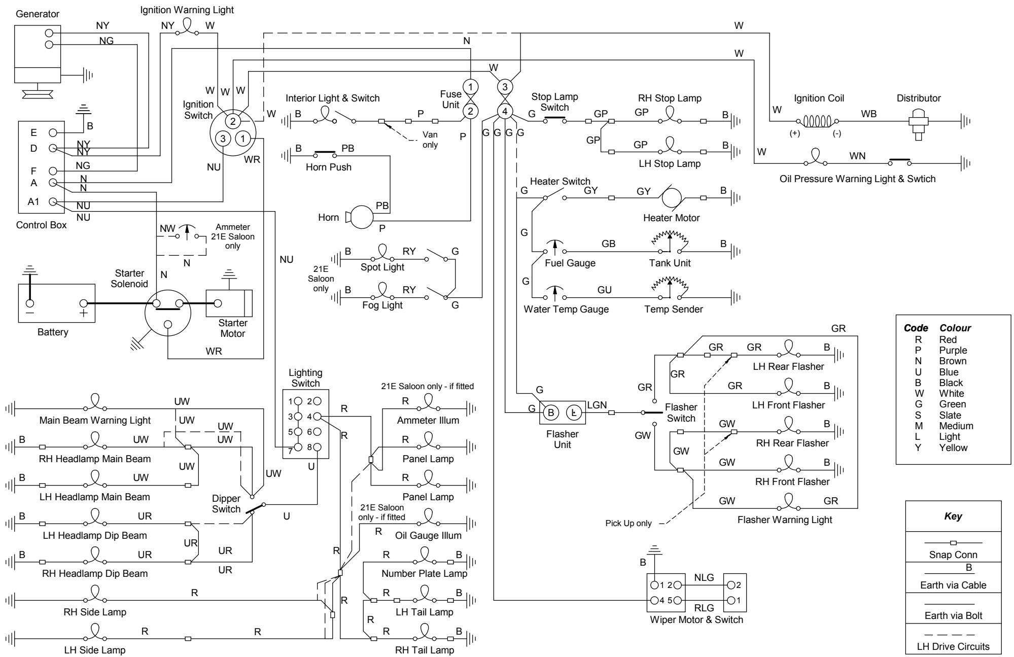
Wiring Diagram - Reliant Regal 3.30 700cc
