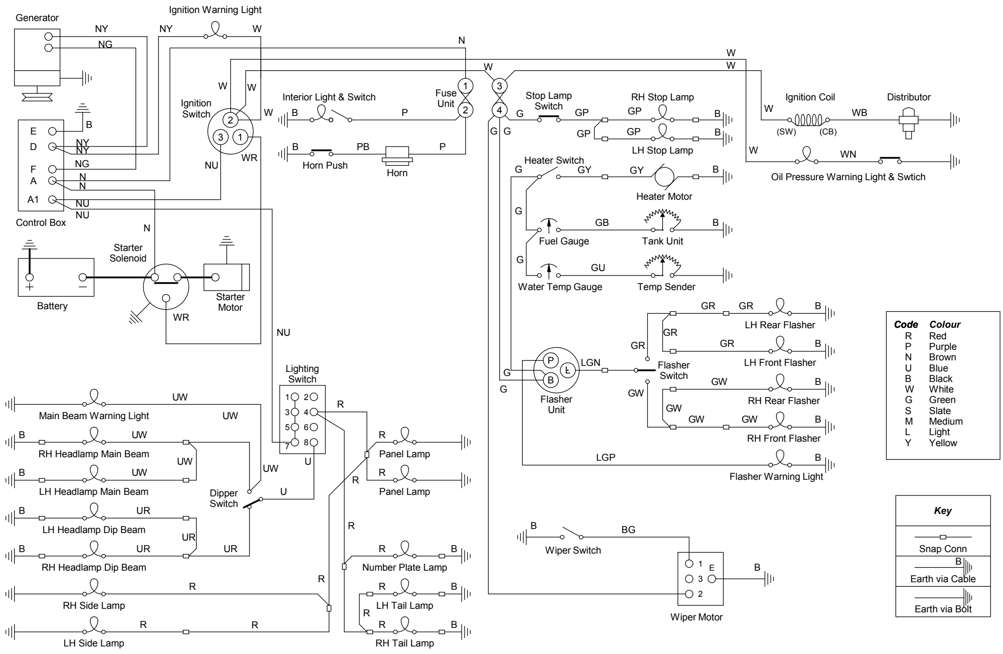
Wiring Diagram - Reliant Regal 3.25 600cc
