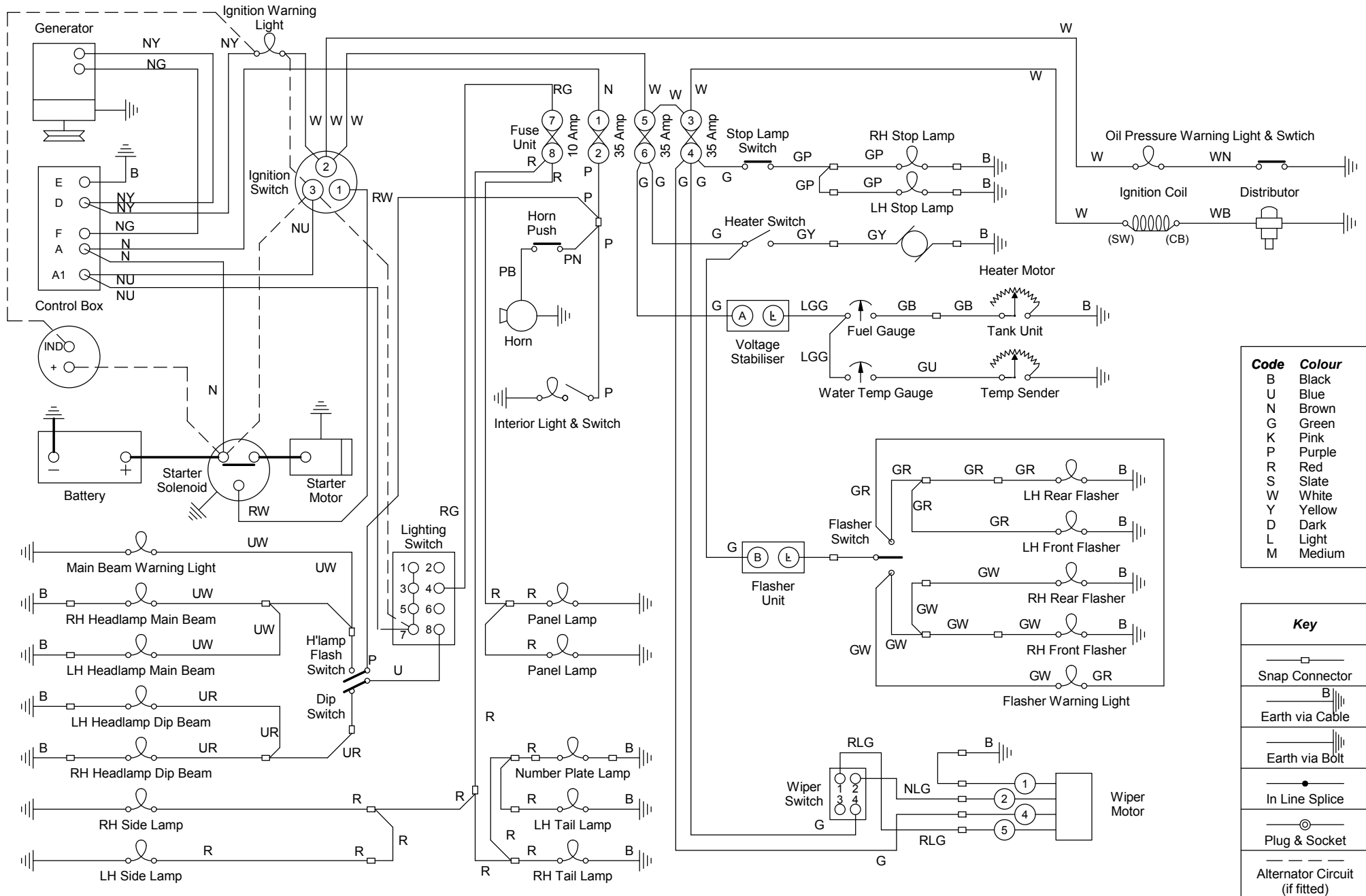
Wiring Diagram - Reliant Rebel
