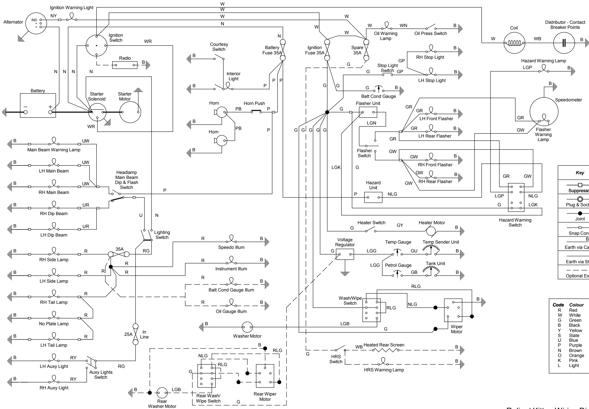
Reliant Kitten Wiring Diagram
