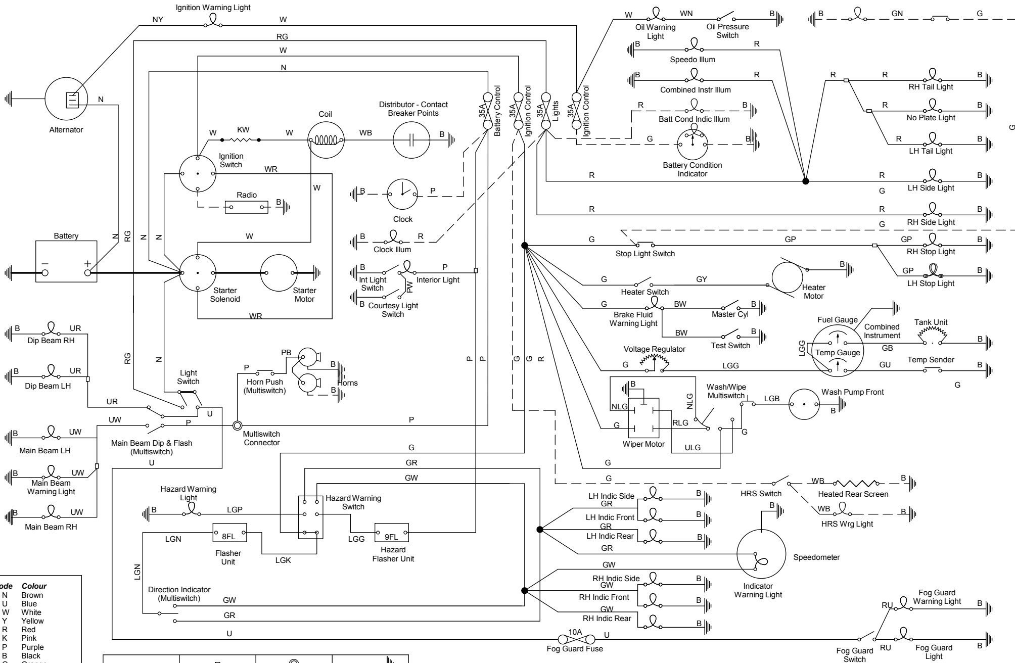
Reliant Fox Wiring Diagram
