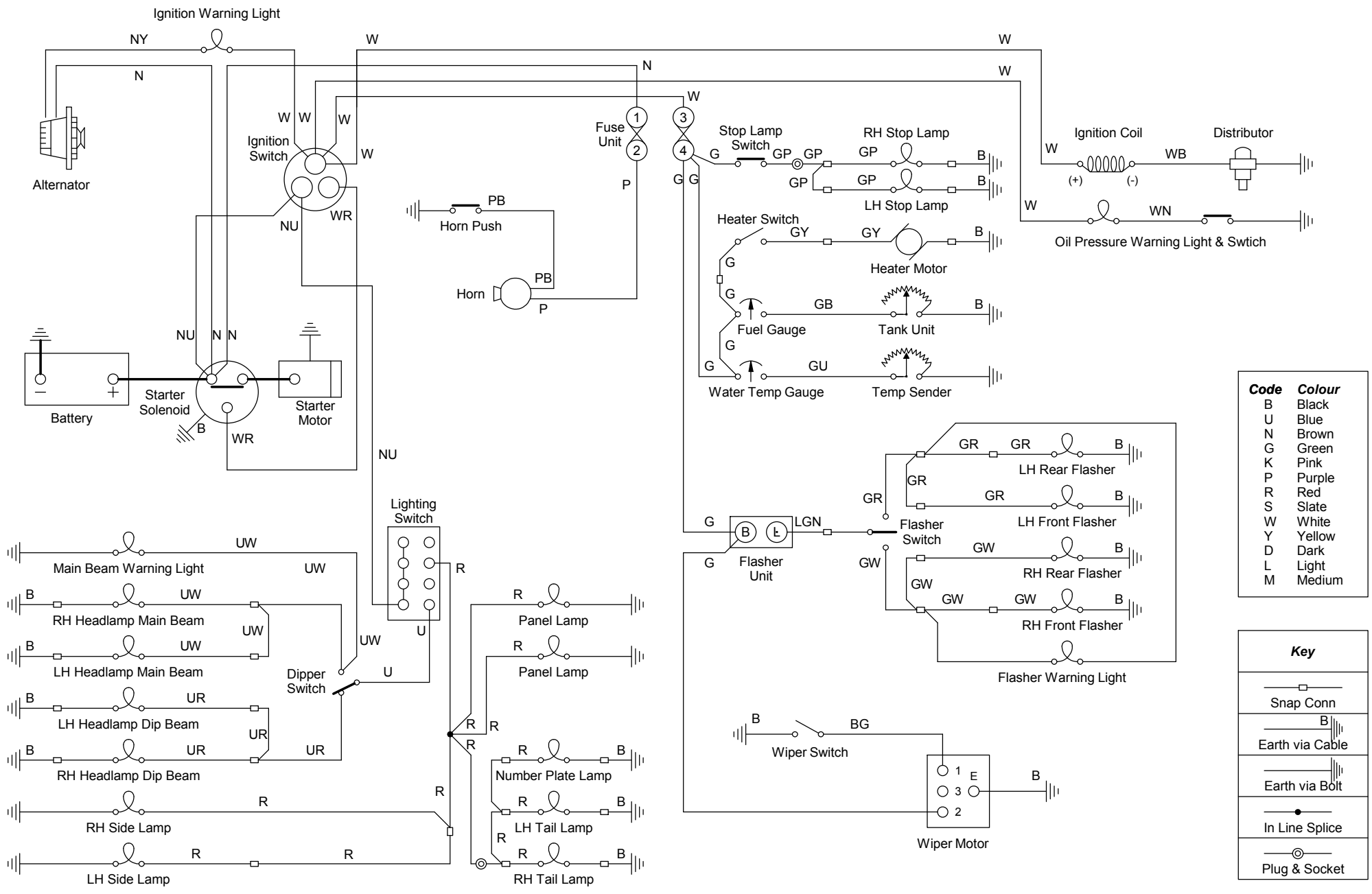
Wiring Diagram - Reliant Ant
